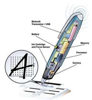
Figure 31: Anoto digital pen and the paper dot pattern.
